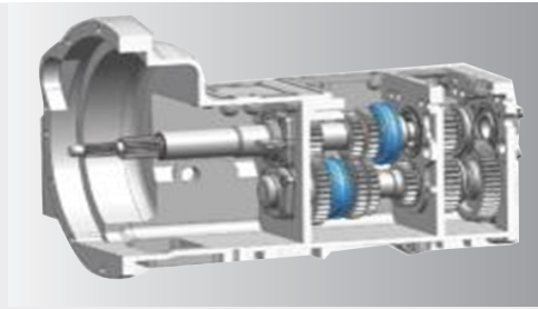
12+12 shuttle gears
